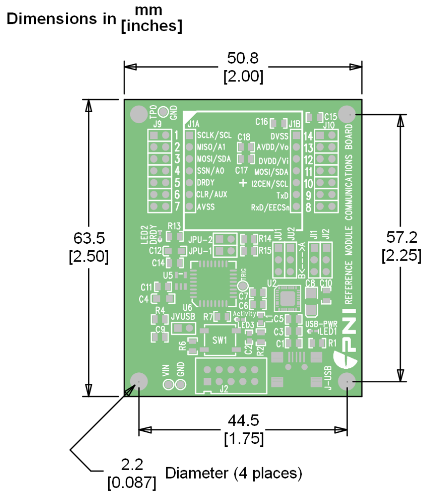
Figure 3-1: CommBoard Top View
